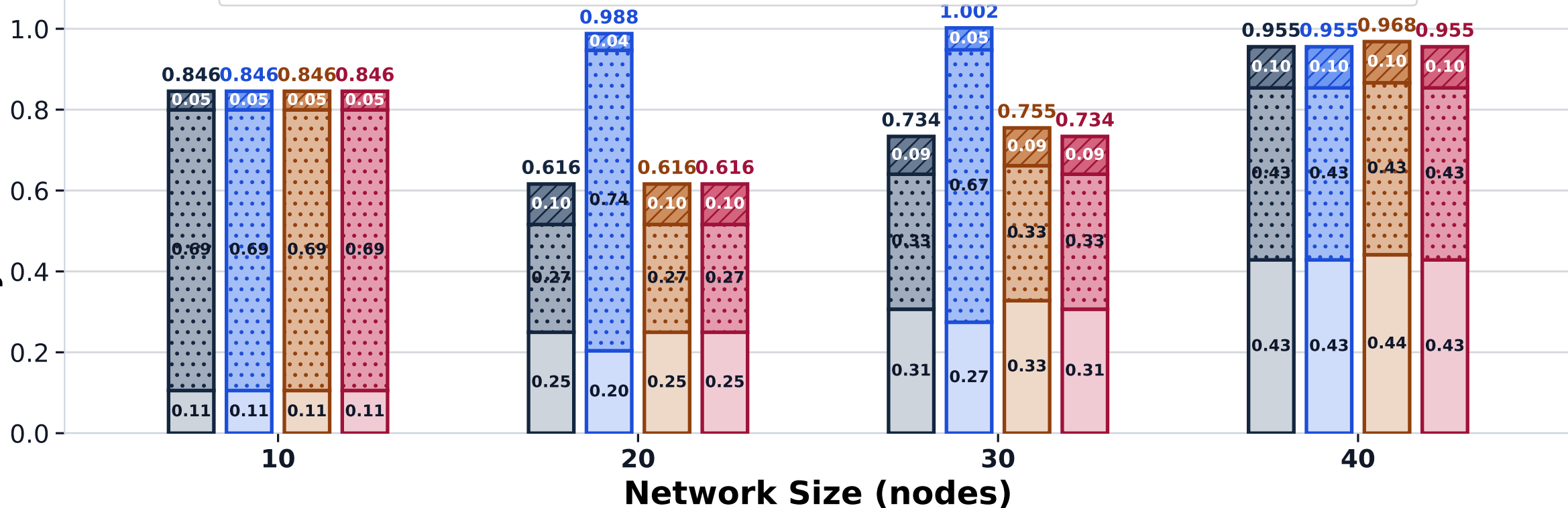
Objective Value
